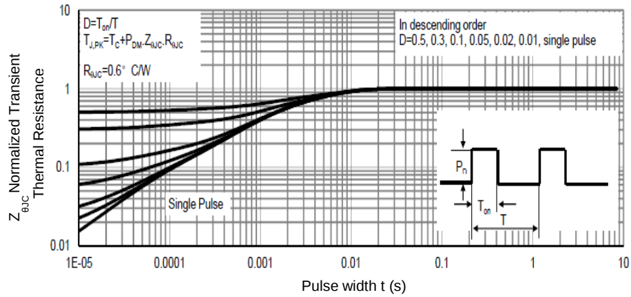
Figure 12. Transient Thermal Response Curve
