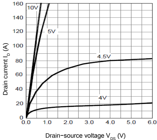
Figure 1. On-Region Characteristics
